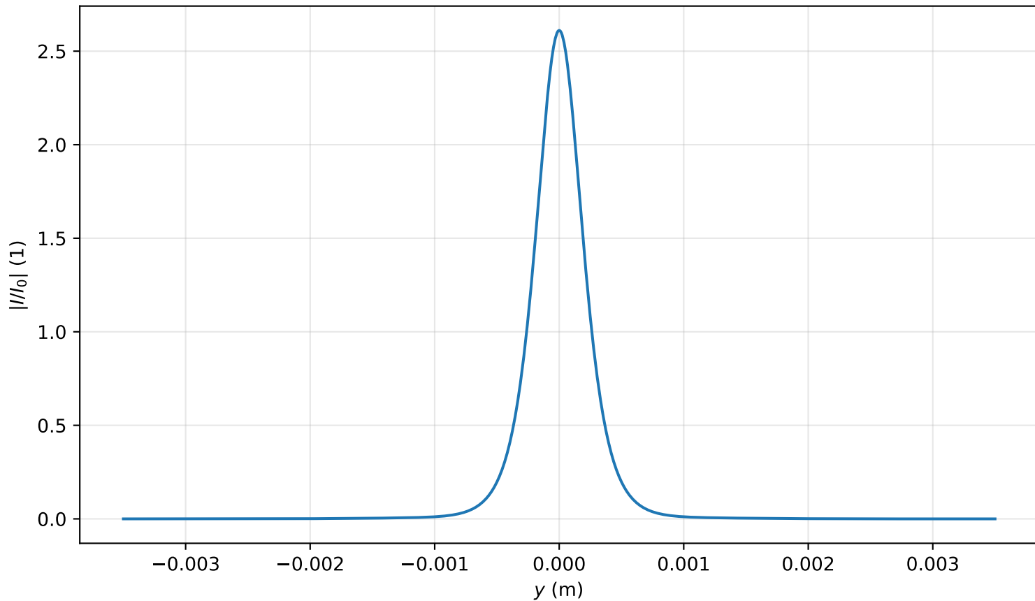
Intensity profile I(x=0, y, z=2.946)/I_0 , \text{Pin}=1.0\text{Pcr} , artificial time
